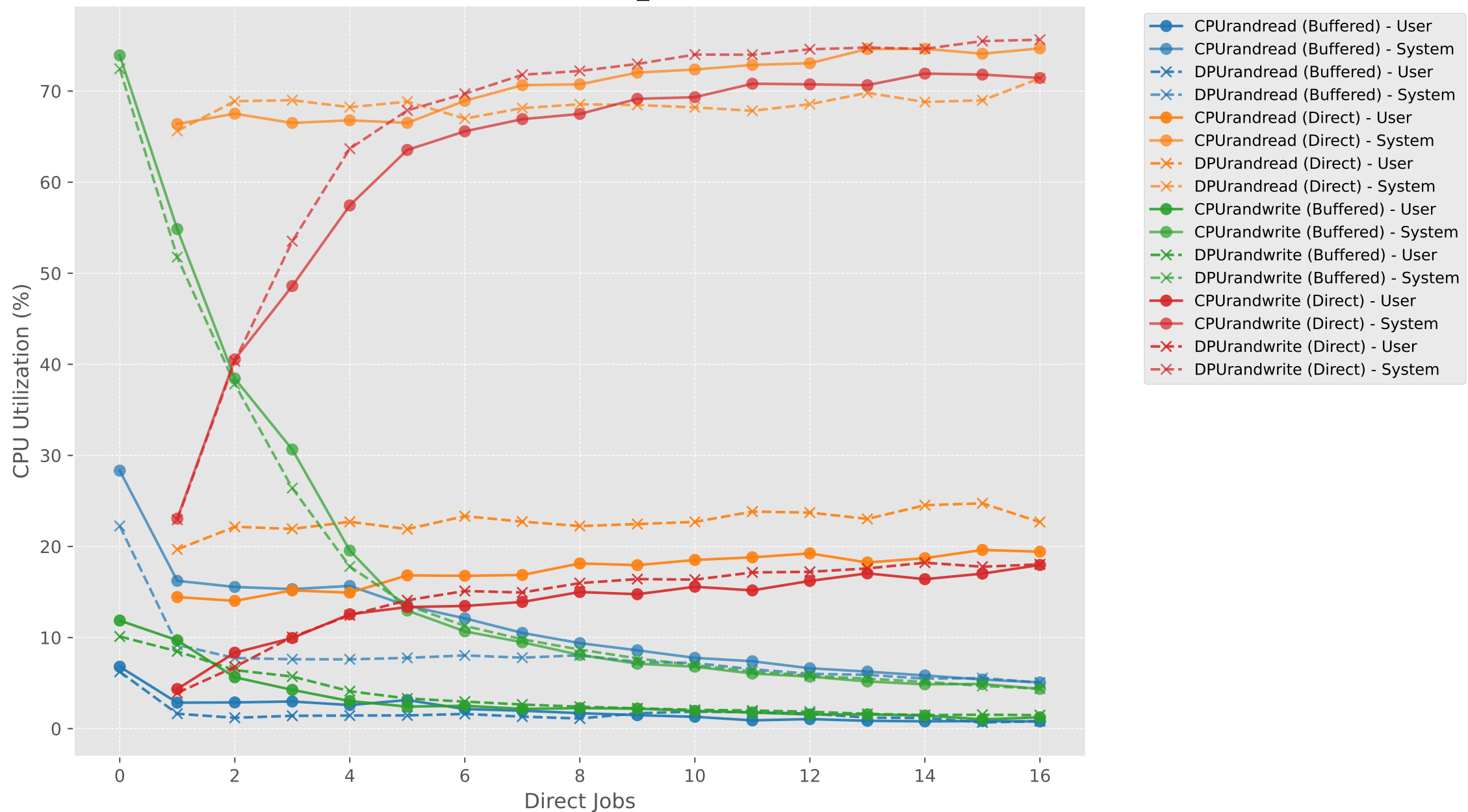
CPU Utilization vs Direct Jobs (buffered1_directN) - RAND (CPU vs DPU)
